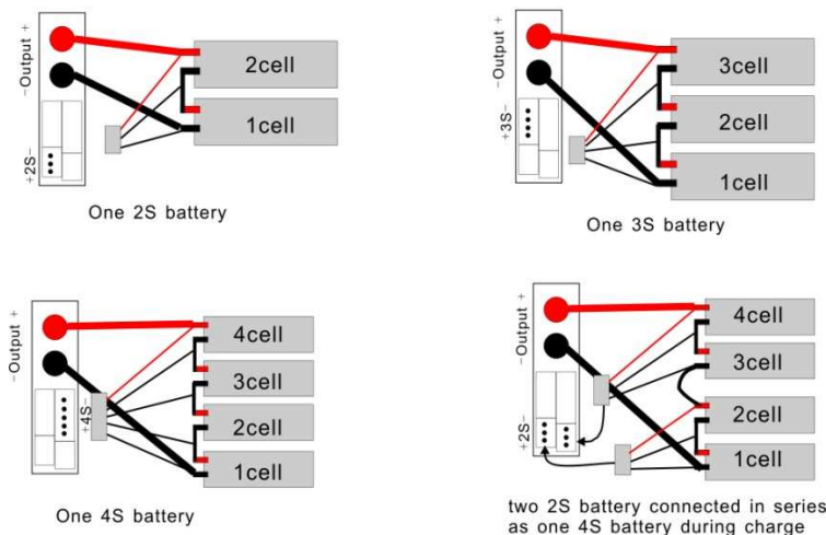
Charging Connection diagram for CHARGERY 0410B
